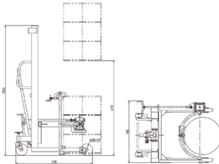
ASSEMBLY DRAWING
